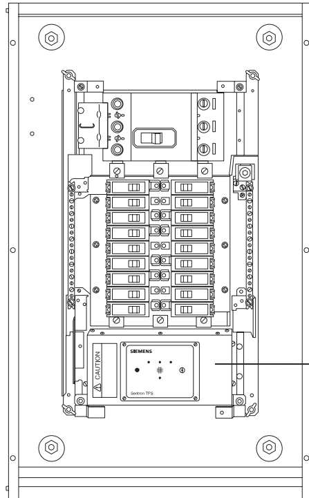
TPS with LED indicators, audible alarm with silence switch, and test button.
