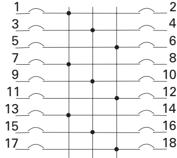
NEMA Numbering
