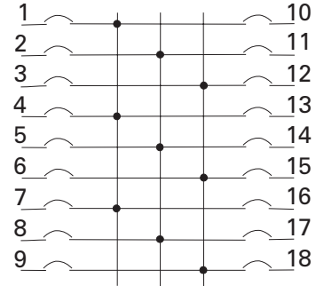
Vertical Numbering
